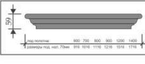
КАРНИЗ №62/1
